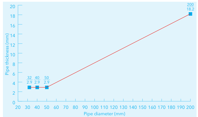
Plastic pipes PP according to EN 1451, U/C, Floor ≥ 150mm - E 120, EI 90
