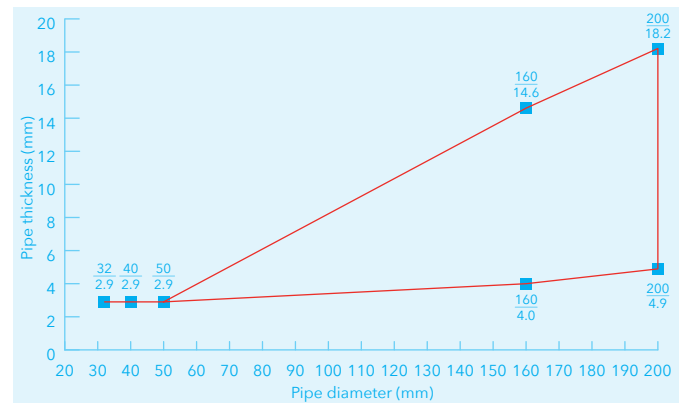
Plastic pipes PP according to EN 1451, wall ≥ 100mm - E 120, EI 90
