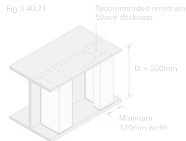
Fig 3.40.21 Full depth nogging or T-nogging For web depths greater than 500mm, contact Promat Technical Services Department.
